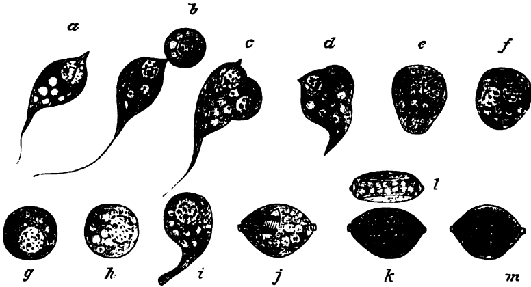
FIG. 33.—Biseual pairing of Stylorhynchus . a , Spermatozoon; b-e , fusion of cytoplasm of spermatozoon and oosphere; f , g , fusion of nuclei; h-j , development of wall to zygote; k , l , formation of four sporoblasts; l , side view of spore; m , mature sporozoites in spore. (After Léger.)
